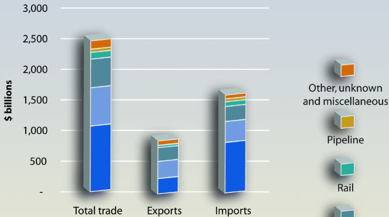
FIGURE 2-2M. U.S. INTERNATIONAL MERCHANDISE TRADE BY MODE OF TRANSPORTATION: 2005
