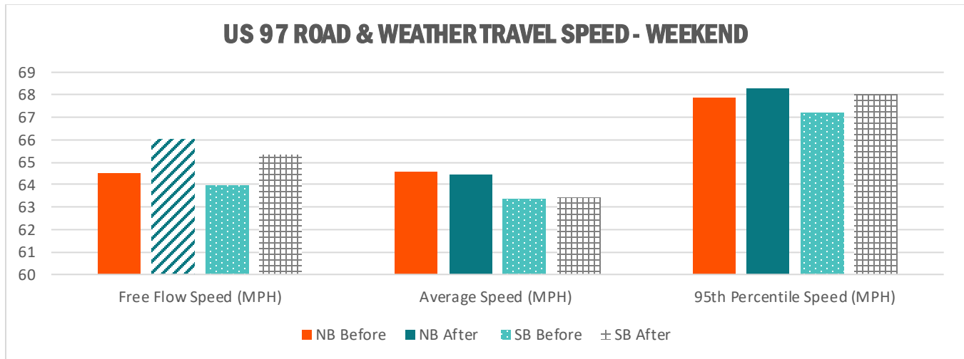
FIGURE 7.6: US97 SPEED PERFORMANCE MEASURES FOR NB AND SB DIRECTIONS DURING WEEKEND PEAK HOURS
