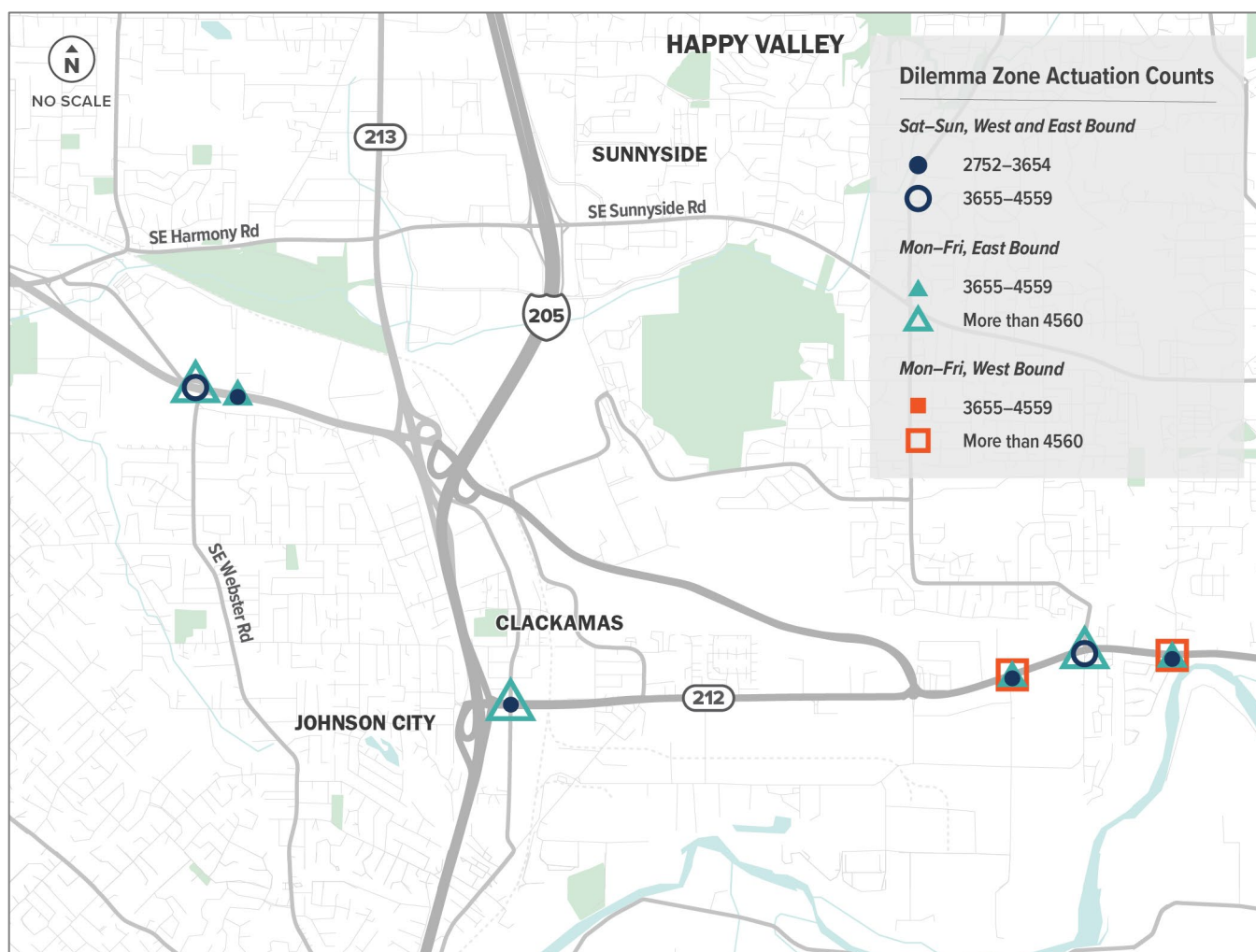
FIGURE 3.155: TOTAL NUMBER OF ACTUATIONS PER WEEKDAY AND WEEKDAY, BY DIRECTION OF TRAVEL
