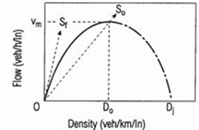
FIGURE 2.2: GENERALIZED RELATIONSHIP BETWEEN FLOW AND DENSITY ON UNINTERRUPTED FLOW FACILITIES
