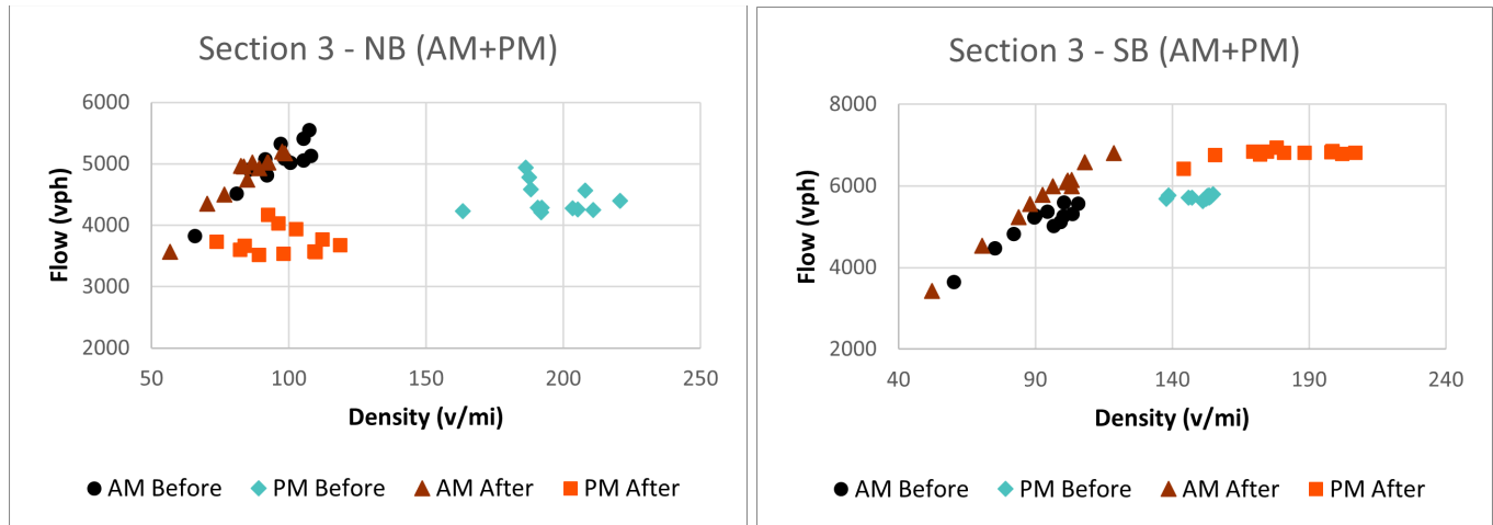
FIGURE 2.5: SECTION 3 FLOW AND DENSITY SCATTER PLOT
