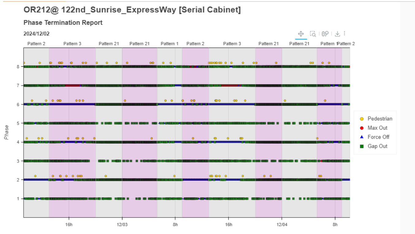
FIGURE 3.111: PHASE TERMINATION REPORT
