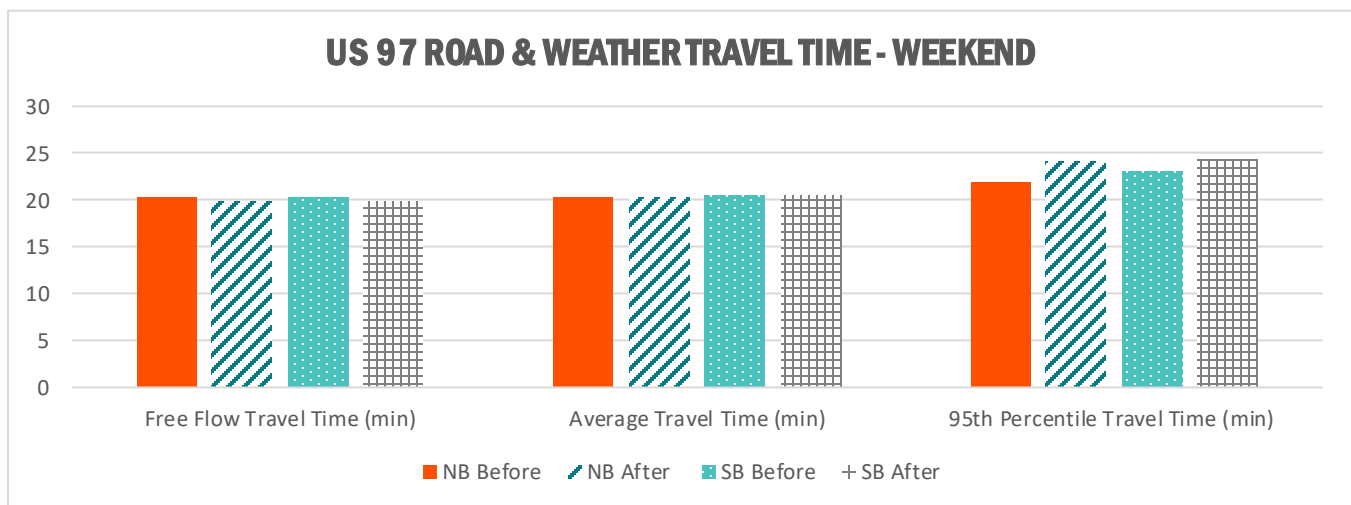
FIGURE 7.7: US97 TRAVEL TIME PERFORMANCE MEASURES FOR NB AND SB DIRECTIONS DURING WEEKEND PEAK HOURS
