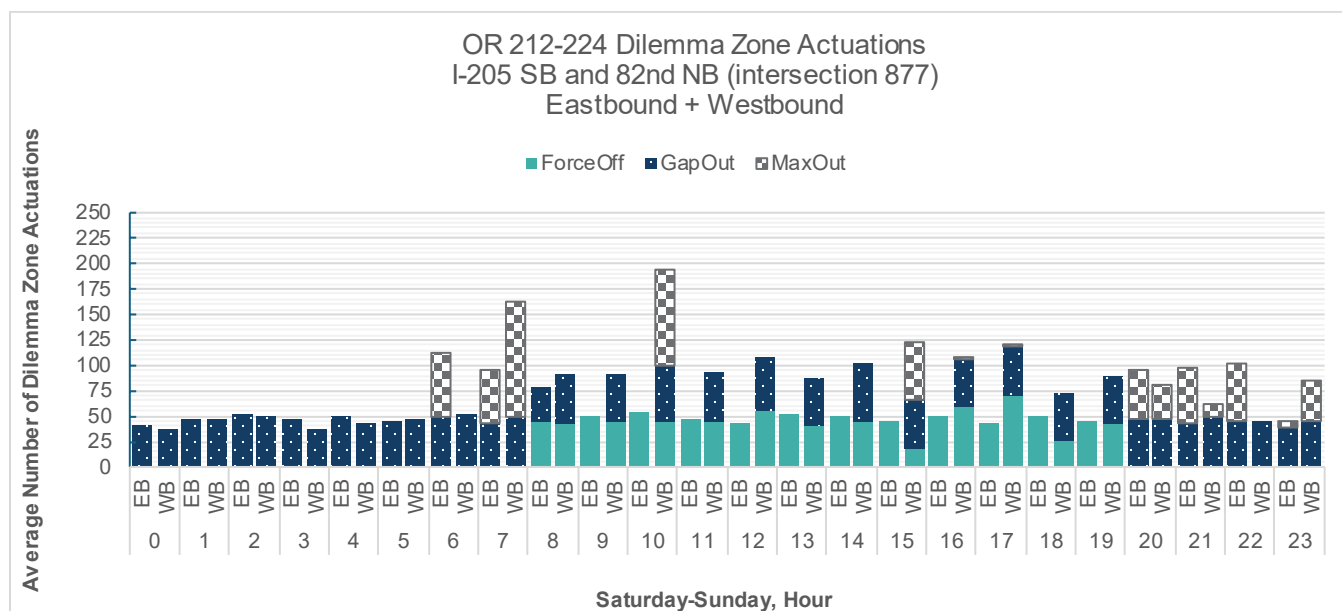
FIGURE 3.144: WEEKENED DILEMMA ZONE ACTIVATIONS ALONG OR 212/224 AND 82ND DR
