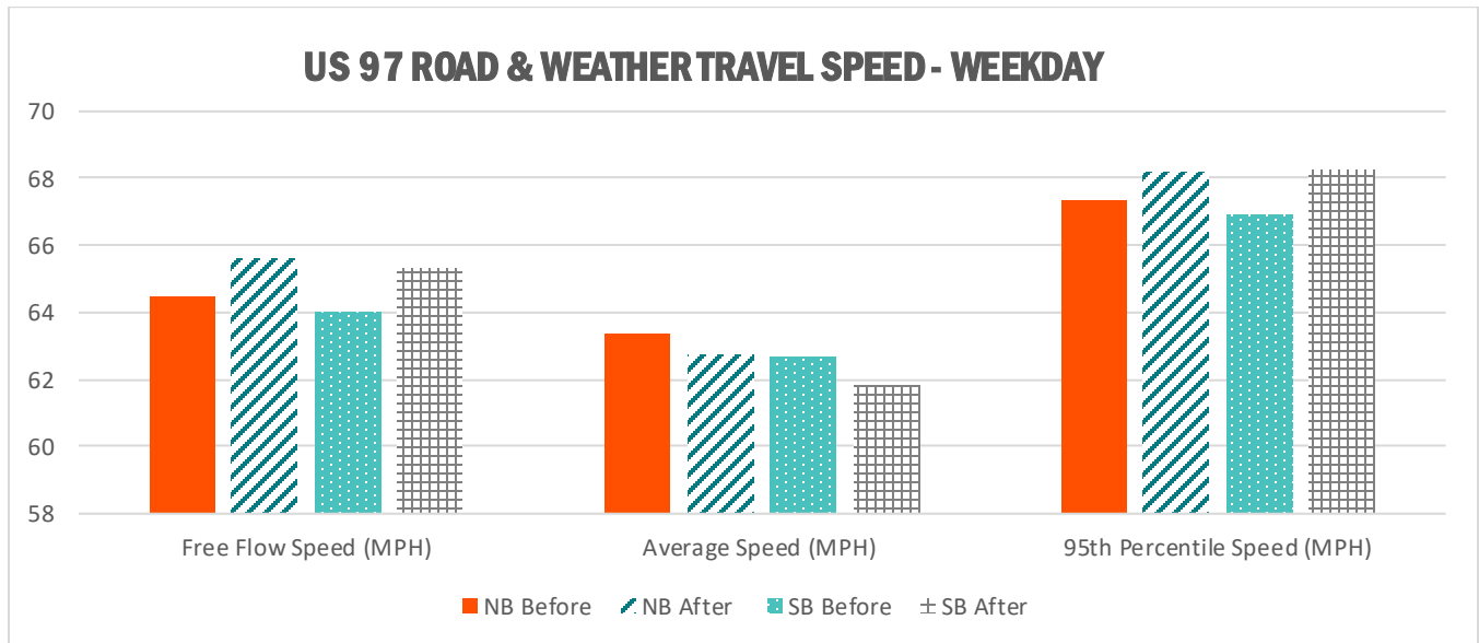
FIGURE 7.4: US97 SPEED PERFORMANCE MEASURES FOR NB AND SB DIRECTIONS DURING WEEKDAY PEAK HOURS
