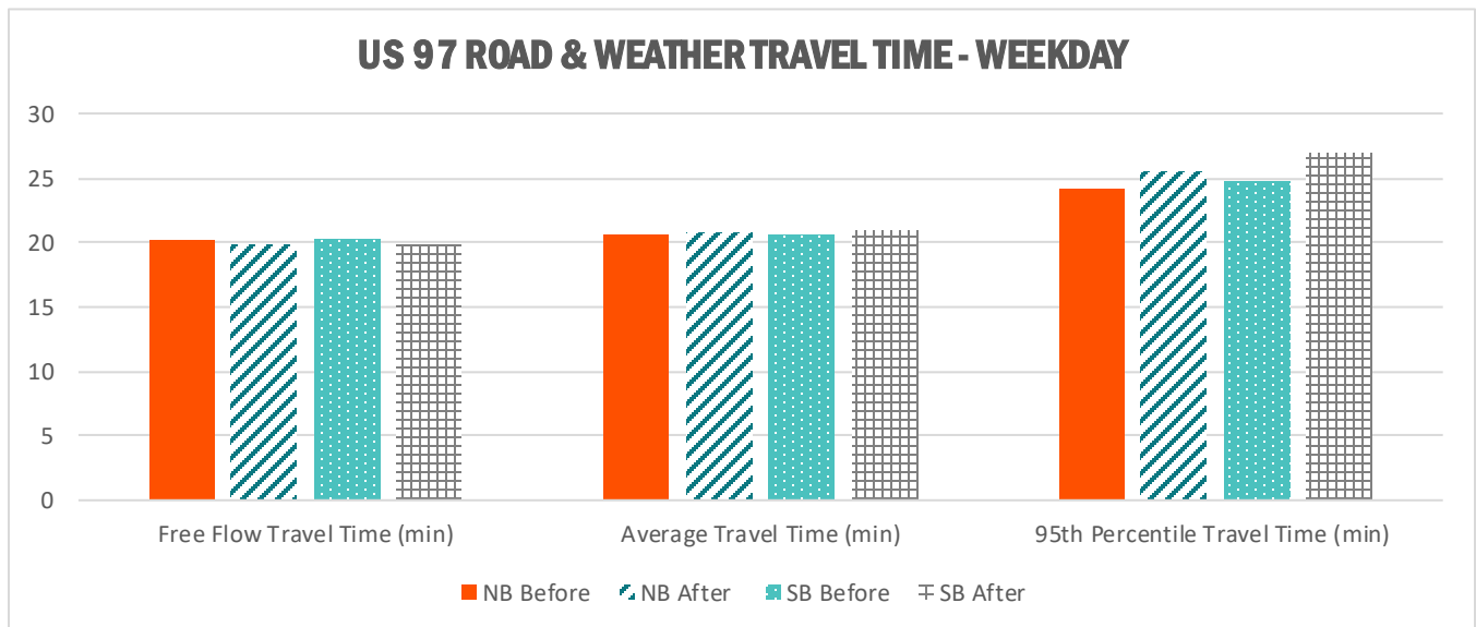
FIGURE 7.5: US97 TRAVEL TIME PERFORMANCE MEASURES FOR NB AND SB DIRECTIONS DURING WEEKDAY PEAK HOURS
