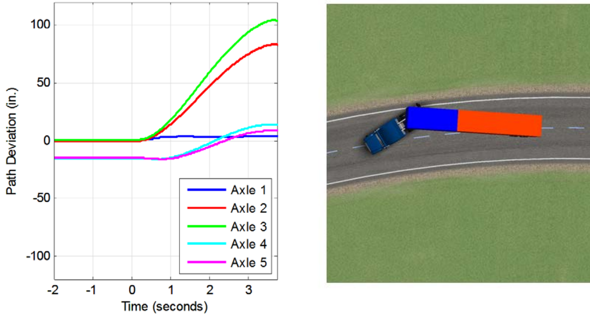
Figure 12: A Bird's Eye View of Control Vehicle CS after Coming to Rest in the Brake-in-a-curve Maneuver with the ABS Disabled on the Drive Axles
