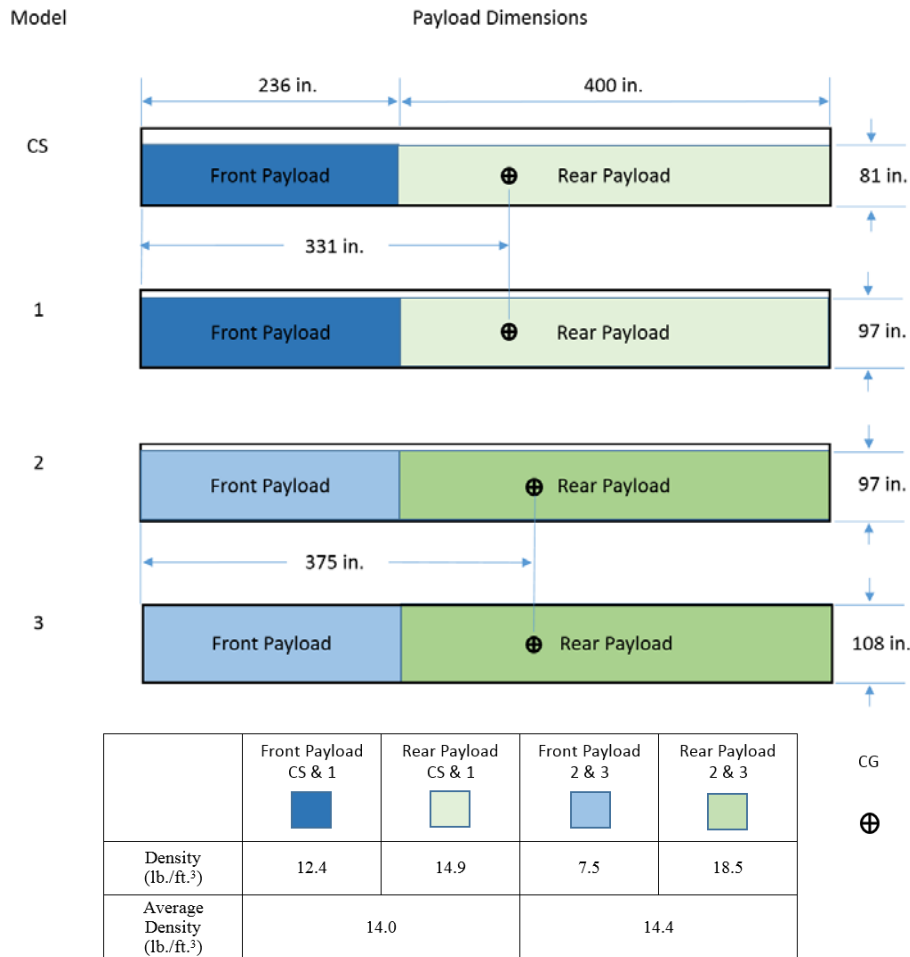
Figure D1. Dimensions of Payloads on the Single-Trailer Combinations
