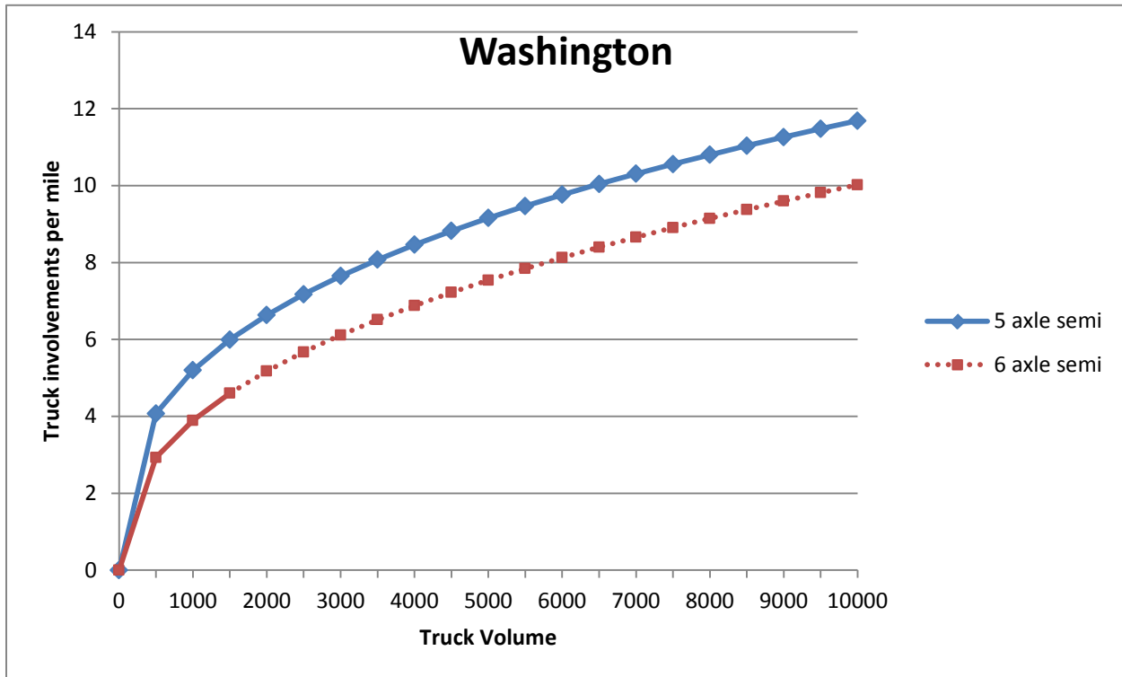
Figure 3: Truck Involvements per Mile versus Truck Volume for Six-Axle Alternative Truck Configurations and Five-Axle Controls in Washington.
