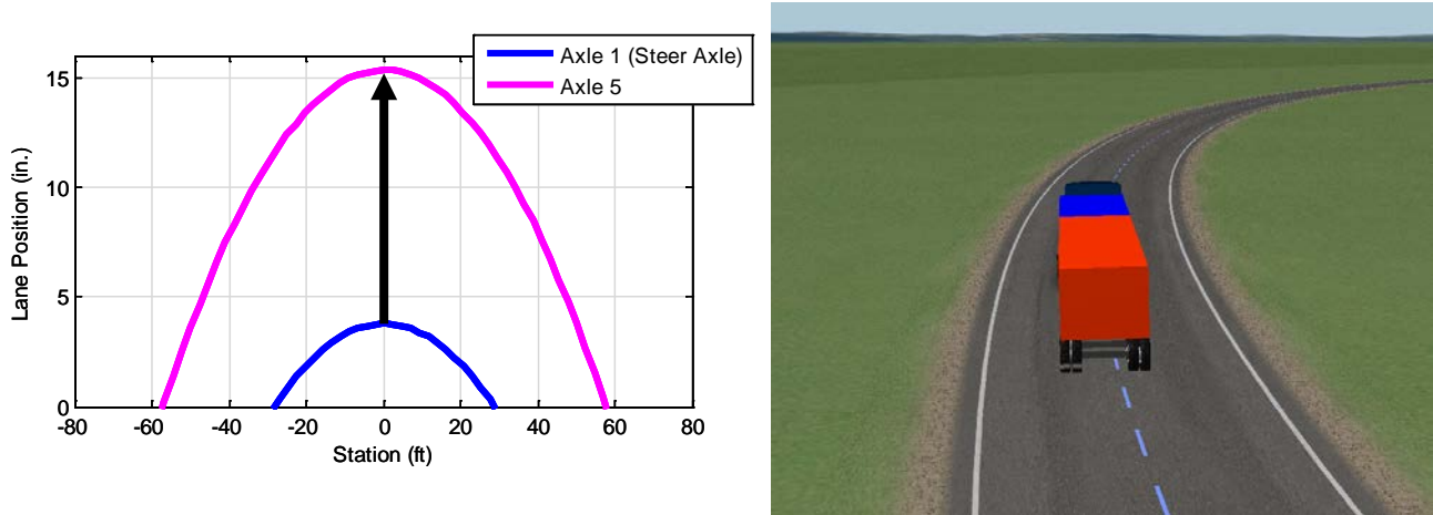
Figure 9: Off-tracking was Calculated by Taking the Difference in the Path Followed by the First and Final Axles.
