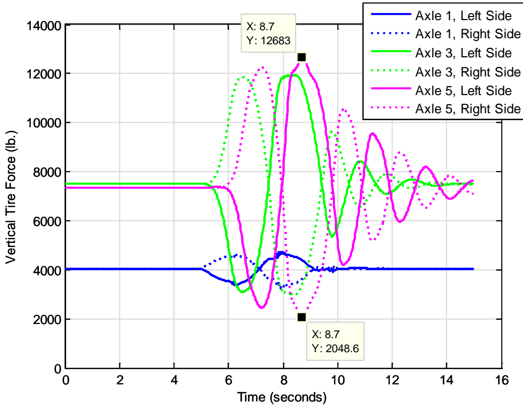
Figure 16: Vertical Tire Forces during the Lane Change Maneuver for the 12-ft Lane Change for Control Vehicle CD 5
