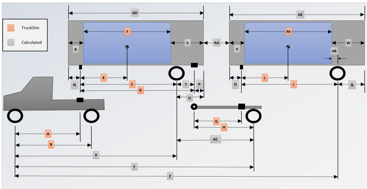
Figure D2. Trailer-to-Trailer Spacing Schematic
