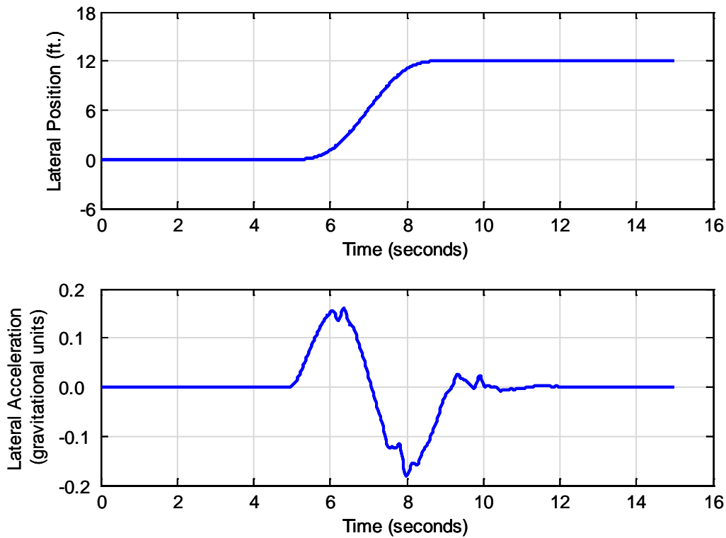
Figure C5. Control Double Vehicle Path While Executing the 12-ft. Lane Change Maneuver
