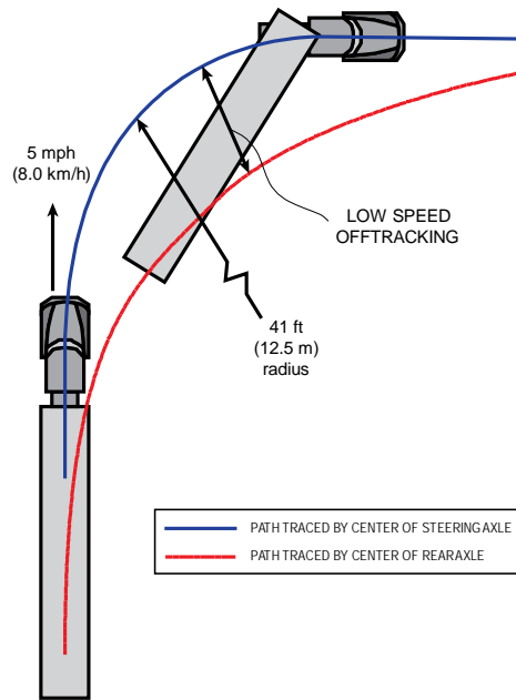
Figure 6: Low-Speed Off-tracking Maneuver Simulates an Intersection
