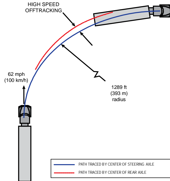
Figure 8: Trailer Tracks to the Outside of the Curve Centerline in this High-Speed Off-tracking Illustration.
