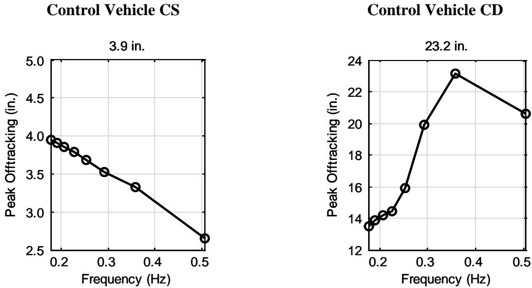
Figure C-7. Maximum Off-tracking for All Excitation Frequencies
