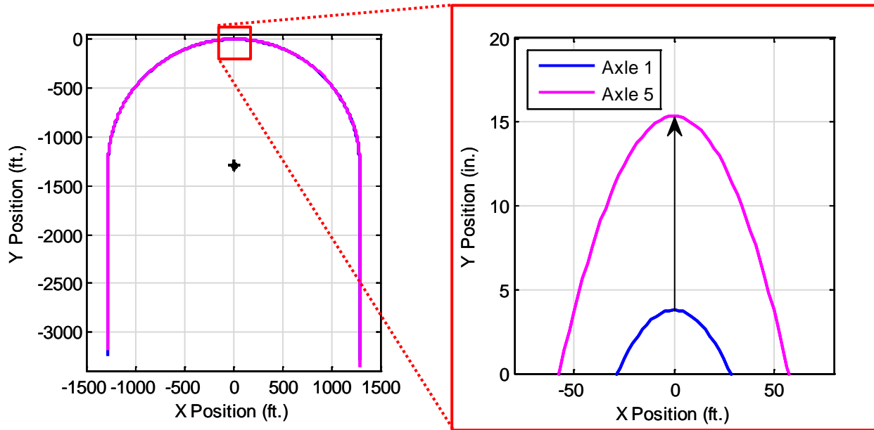
Figure C4. High-speed Off-tracking Path Differences
