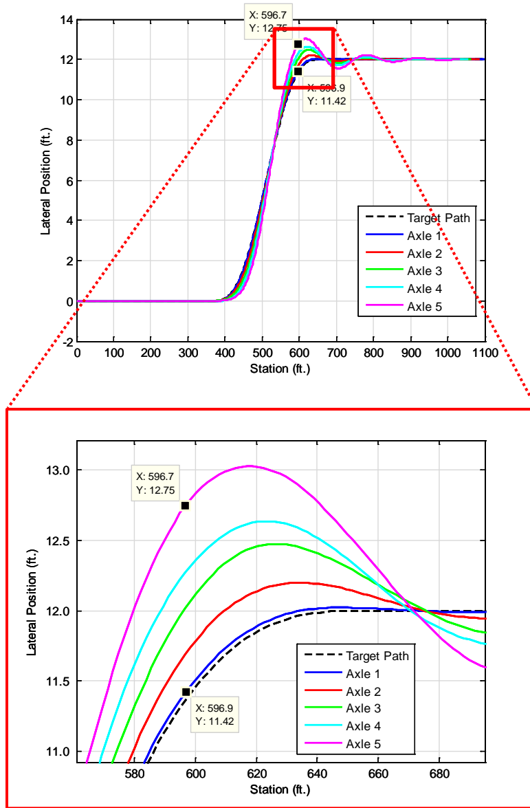
Figure C6. Control Double Vehicle Off-tracking Calculation for the 12-ft. Lane Change
