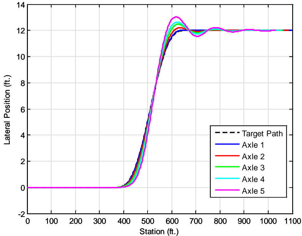
Figure 13: Paths of the Axle centerlines of the Control Double as it Executes the 12-ft. Avoidance Maneuver
