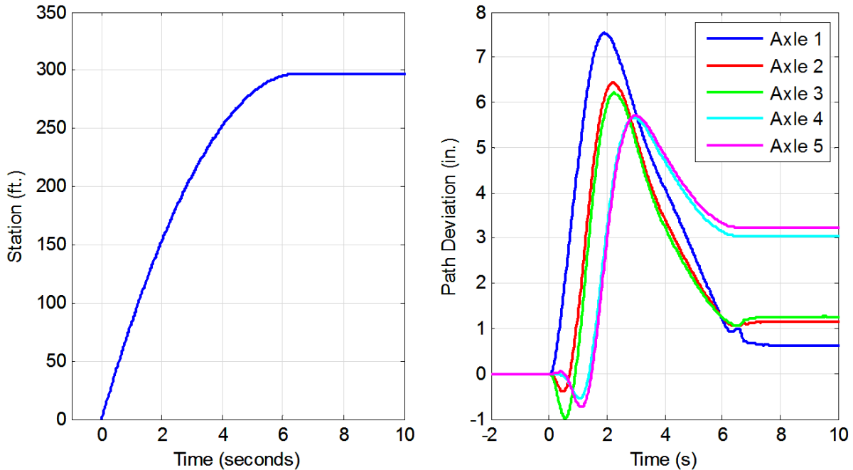
Figure 11: Position vs. Time (left) and Path Deviation vs. Time (right) of Control Single Vehicle as it Stops with Brake Failure on the Right Ends of the Two Drive Axles
