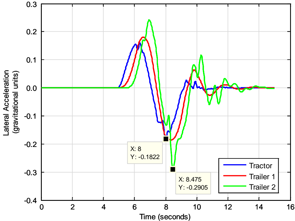
Figure 15: Lateral Acceleration Time Histories of the Three Units of Control Vehicle CD in the 12-ft Lane Change. 4
