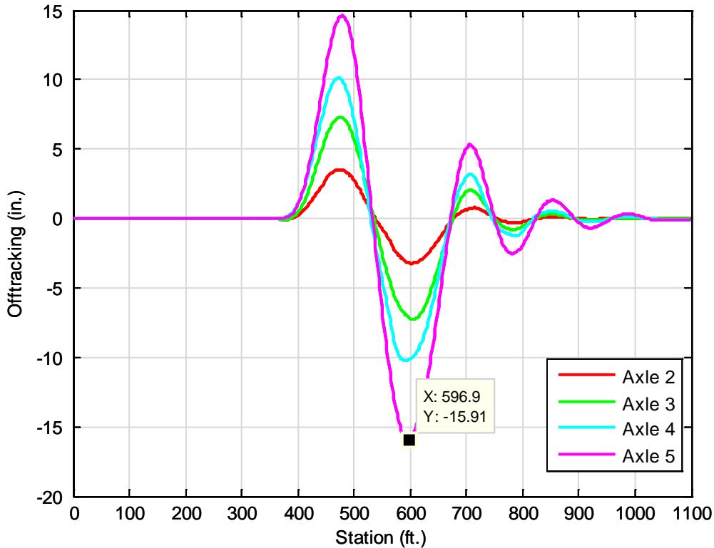
Figure 14: Off-tracking was Computed from the Axle Paths in the Previous Figure 3
