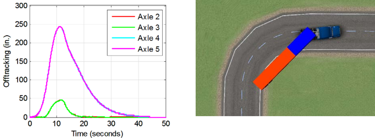
Figure 7: Off-tracking of the Drive and Trailer Axles Rises and Falls During the Maneuver.
