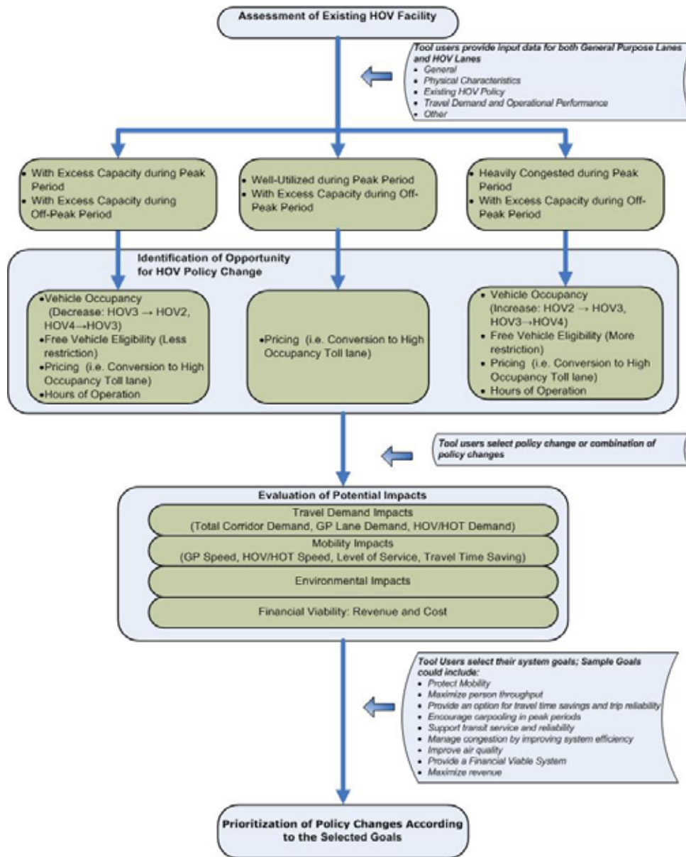
Figure 1: POET-ML Framework
