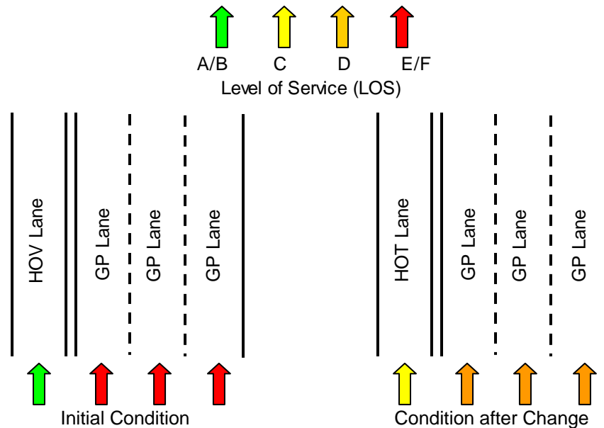
Figure 4: Scenario 2 Lane Condition Diagrams
